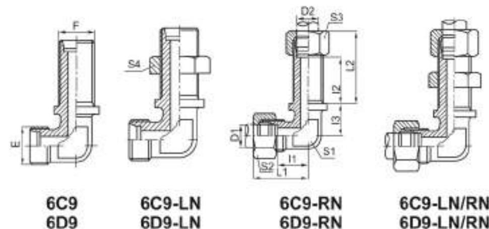
90° 弯曲过板接头 90° ELBOW BULKHEAD FITTINGS
