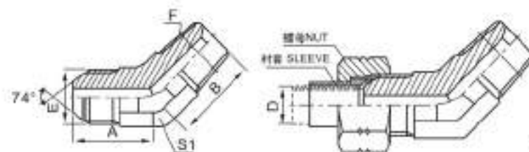
45°弯美制JIC外螺纹74°外锥/英锥管外螺纹 45° ELBOW JIC MALE 74° CONE/BSPT MALE
